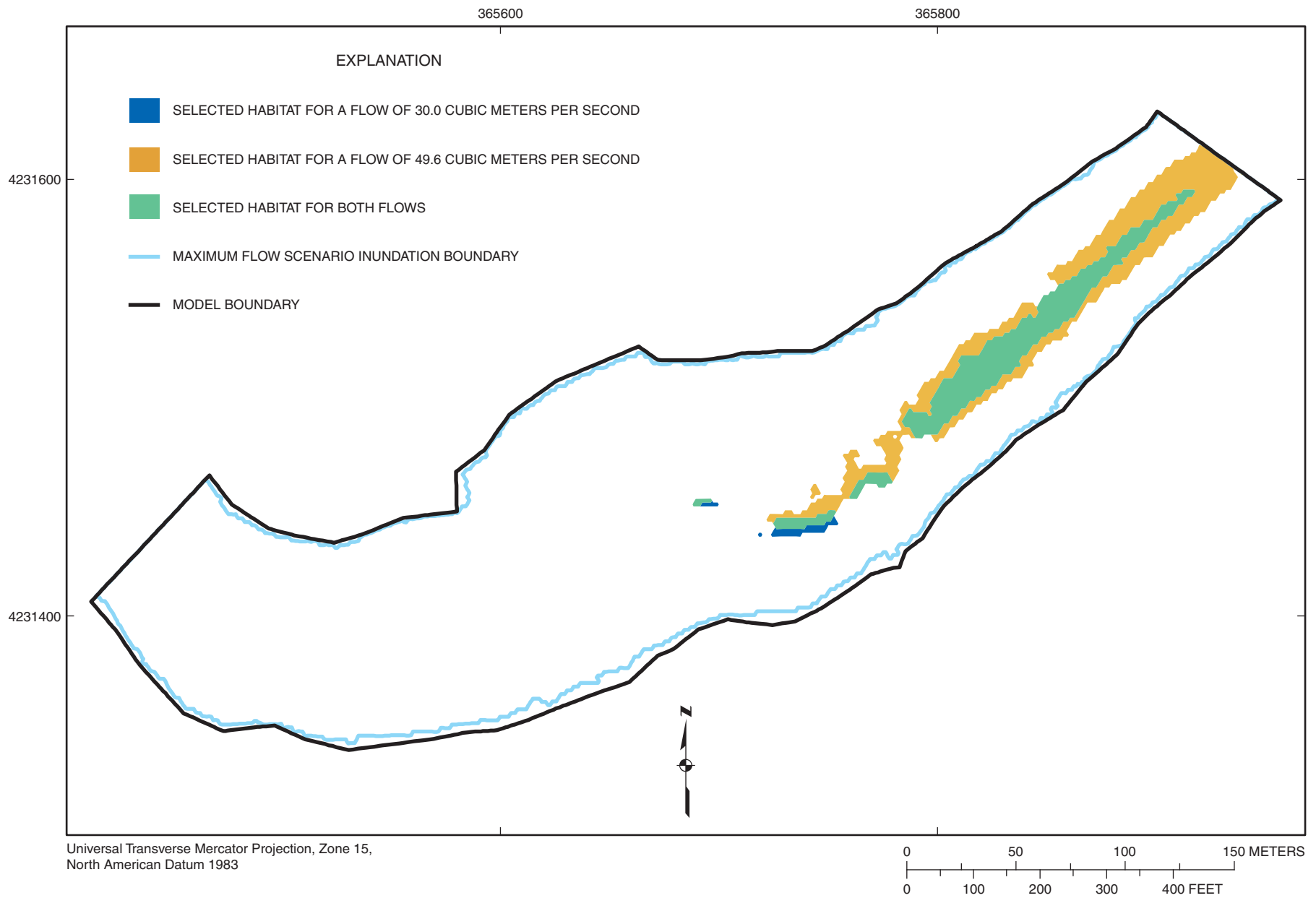
Figure 4-25. Selected habitat area distribution for habitat category 7 (paddlefish) at flows of 30.0 and 49.6 cubic meters per second at Marais des Cygnes River site MDC2.
